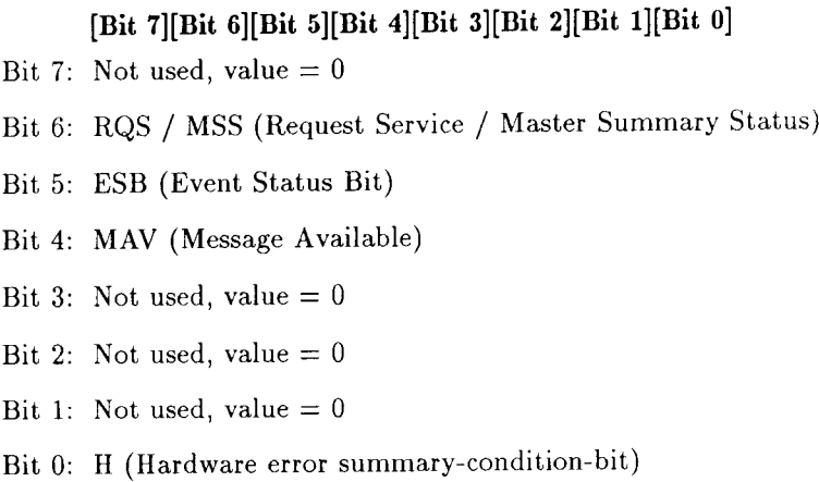
Figure 3-2. Status Byte Register
